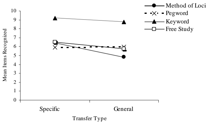
Figure 2 . Specific Vs. General Transfer
